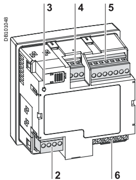
Power Meter Series 700. 1 Mounting slots. 2 RS 485 communications (PM710) or 2 pulse outputs (PM700P). 3 Heartbeat LED. 4 Power supply. 5 Voltage inputs. 6 Current inputs.
